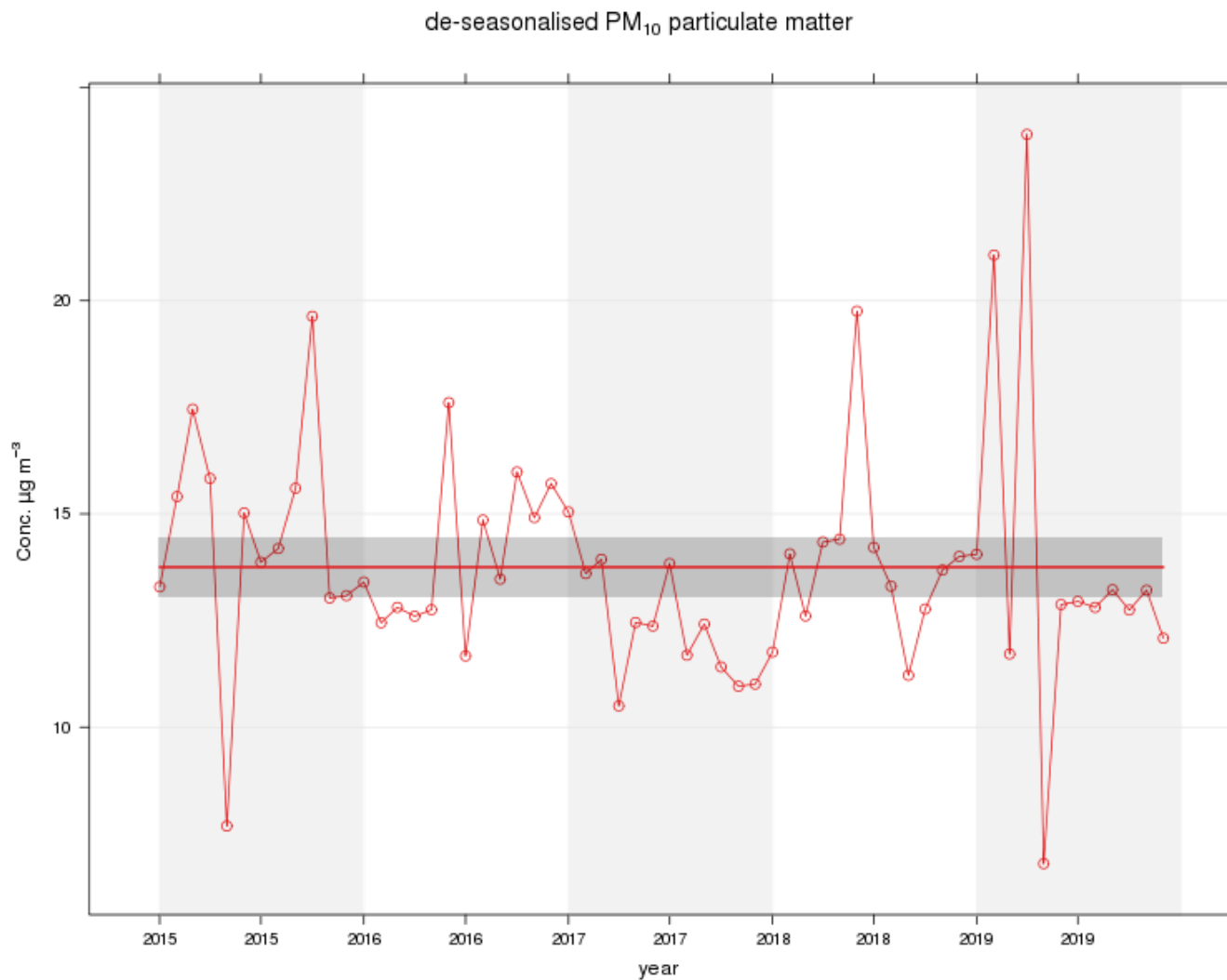
Figure 8 – A4 Hags Long Term PM 10 (24-hour mean) Concentrations
