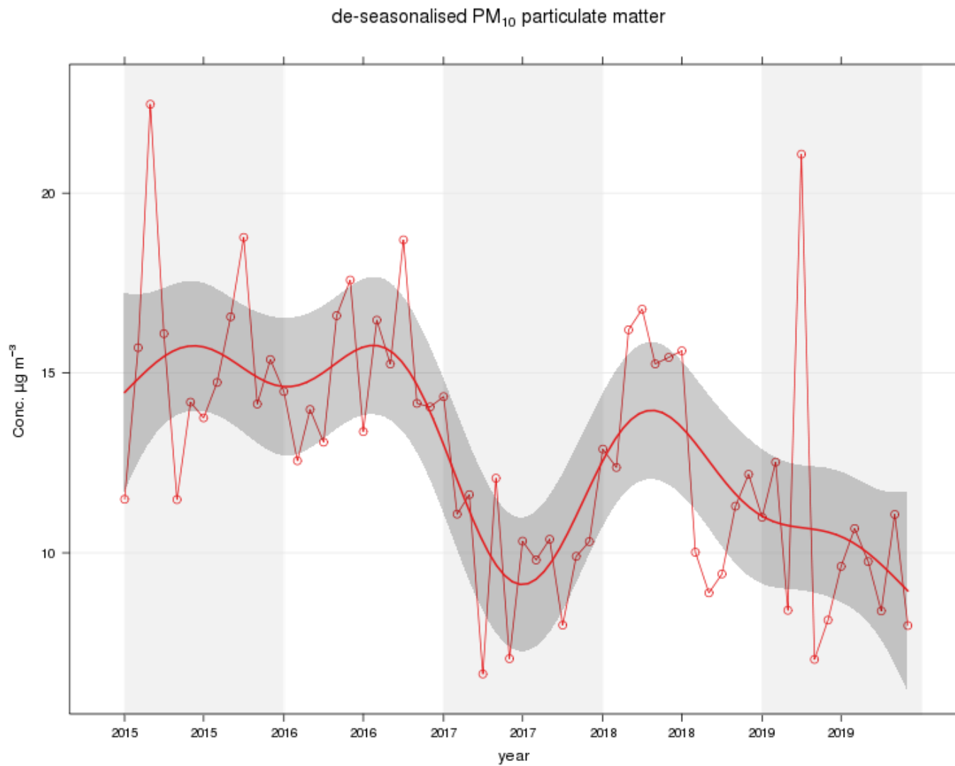
Figure 10 – A7 Falkirk West Bridge St Long Term PM 10 (24-hour mean) Concentrations
