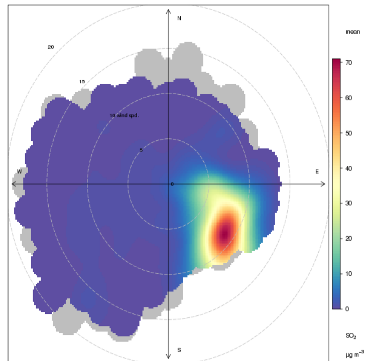
Polar plot of SO 2 at Falkirk Grangemouth MC mean for the period 2015 to 2019
