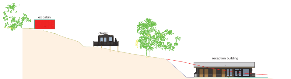
S-21 Section 1:200
