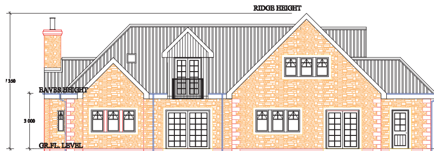
Rear Elevation
