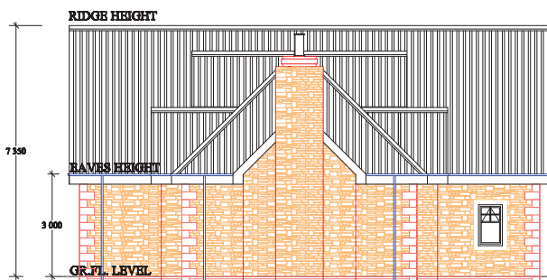
Side Elevation
