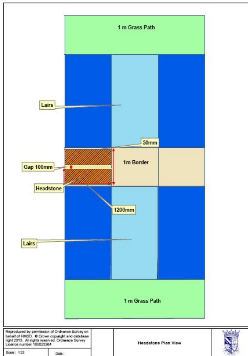
Appendix 11 – dimensions of Memorial Headstone footprint
